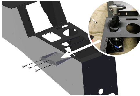
Install shifter/mounting plate assembly to inside of console and into boot. Secure assembly to console with provided (3) socket head cap screws and reconnect wire cord.
