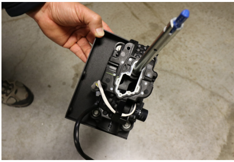
Secure shifter to Mount Plate with factory OEM bolts.
