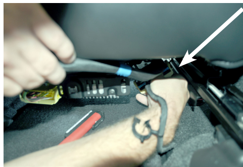
Disconnect wire harness under P/S seat by unlocking the lever, and pulling wire connector apart.
