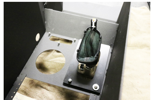
With the console turned over, install the boot and shifter and re-tighten T-20 screws. Snap the boot clips into the Filler Plate.
